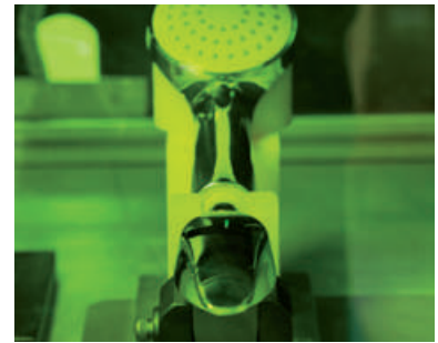
Laser beam during logo engraving process (I).
